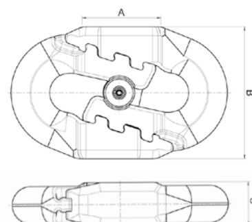
Assembly of chain connector FL
